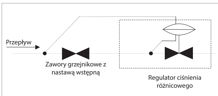
Schemat Frese PV Compact
